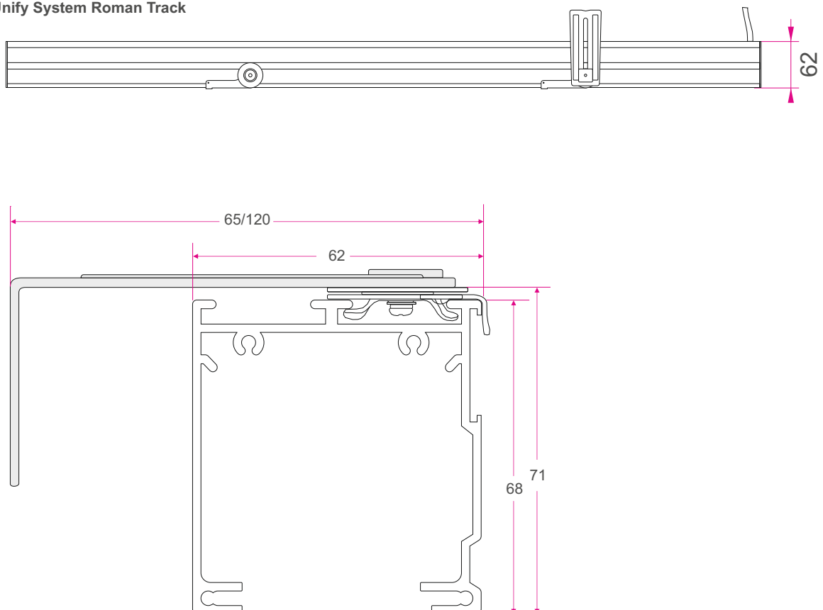
Unify System Roman Track
