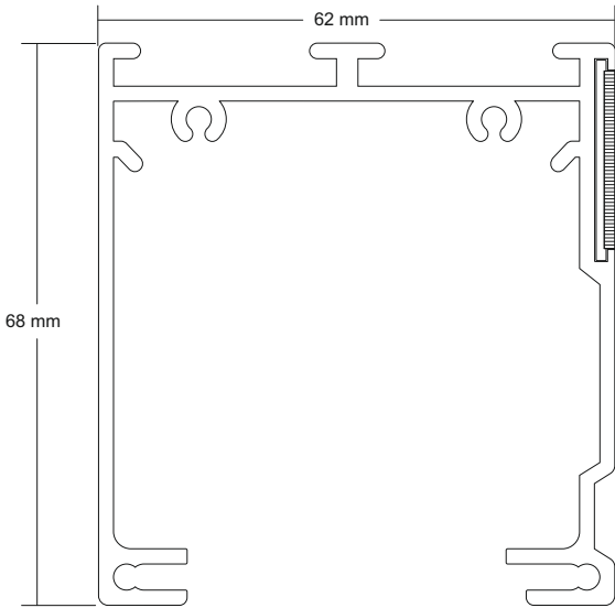
ALUMINIUM TRACK PROFILE
